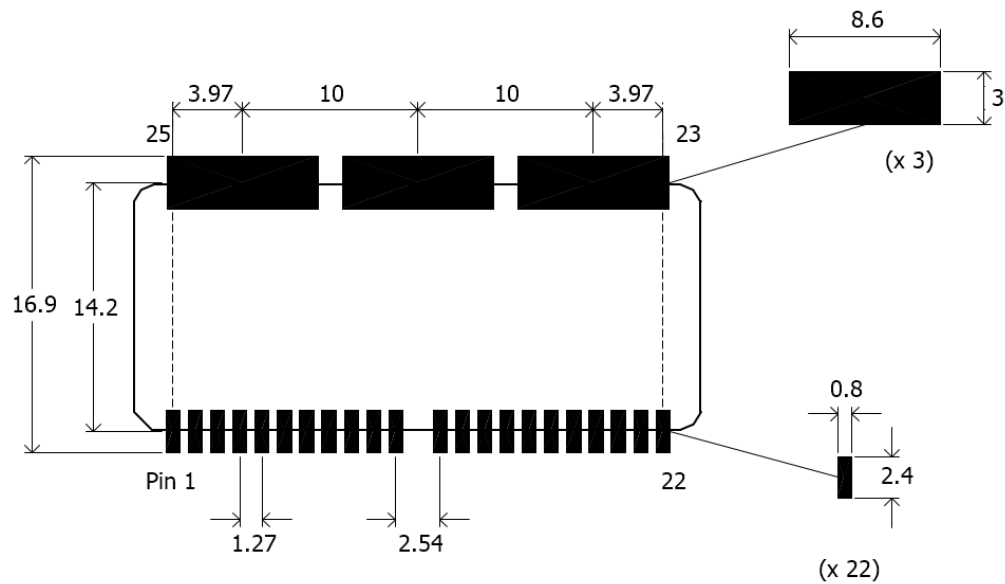
Figure 52. Recommended PCB Pad Sizes
