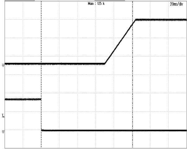
Figure 6: Turn-on transient at full rated load current (constant current load) (20 ms/div). V_{in}=48V . Top Trace: V_{out} , 5V/div; Bottom Trace: ON/OFF input, 2V/div
