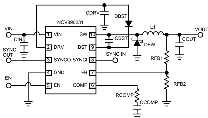
Figure 1. Typical Application
